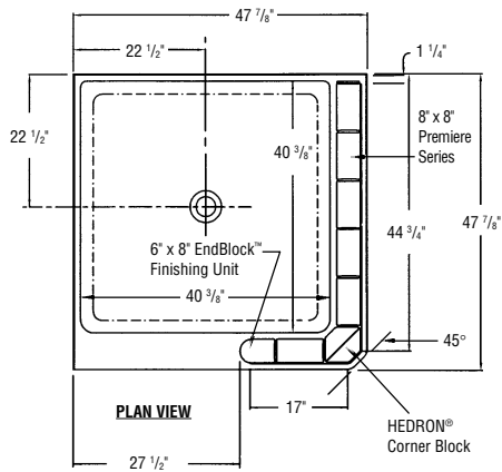
CLASSIC SHOWER FLOOR PLAN (installed with entry on left)
